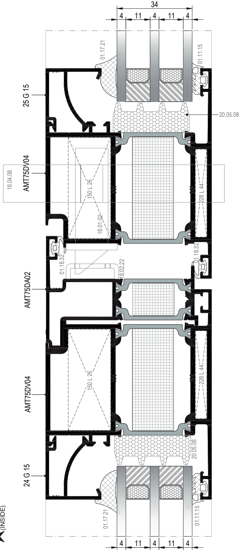
DİŞA AÇILIM ADAPTÖRLÜ HEMYÜZ KAPI DETAYLARI OUTWARD OPENING FLUSH DOOR DETAILS
