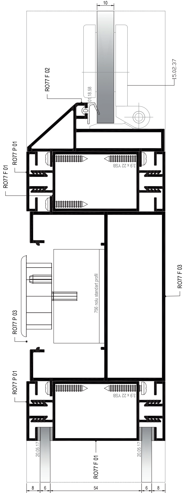
DETAYI 19 DETAIL
