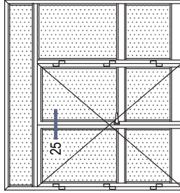
İÇE AÇILIM ADAPTÖRLÜ HEMİYÜZ KAPI DETAYLARI INWARD OPENING FLUSH DOOR DETAILS WITH ADAPTER
