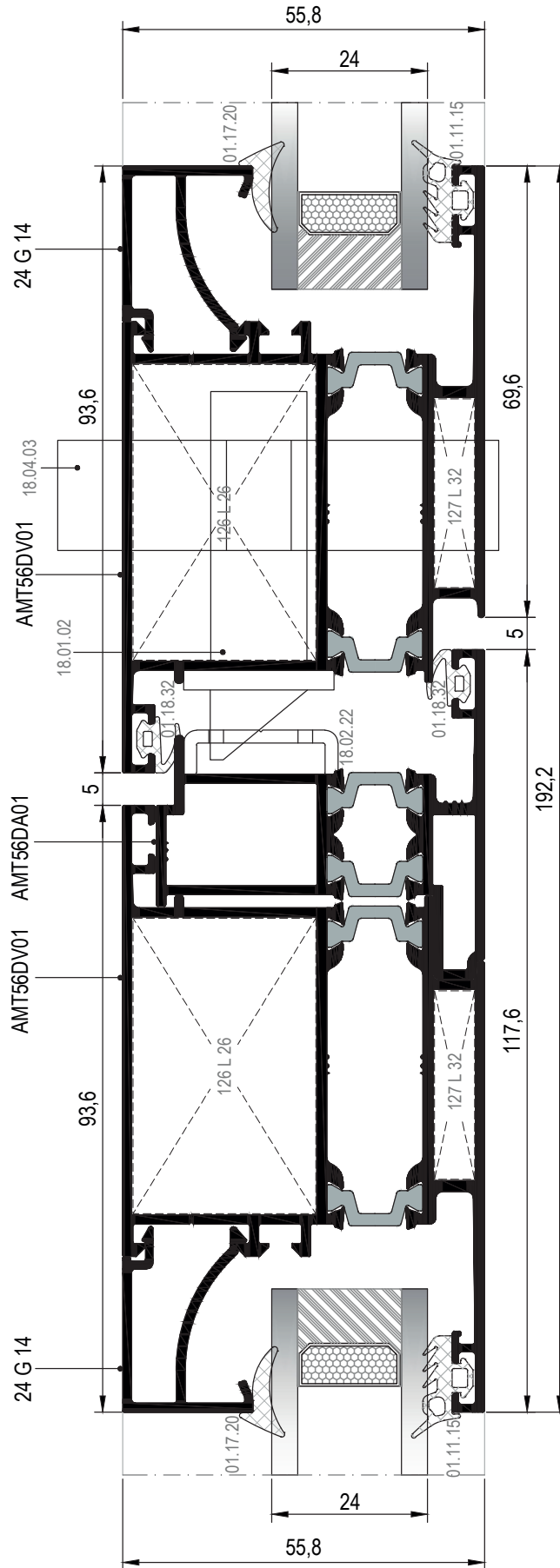
İÇE AÇILIM ADAPTÖRLÜ HEMİYÜZ KAPI DETAYLARI INWARD OPENING FLUSH DOOR DETAILS WITH ADAPTER
