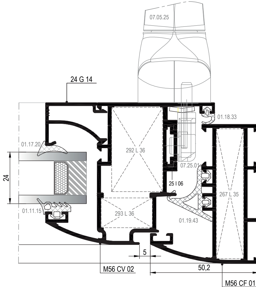
16 DETAYI DETAIL
