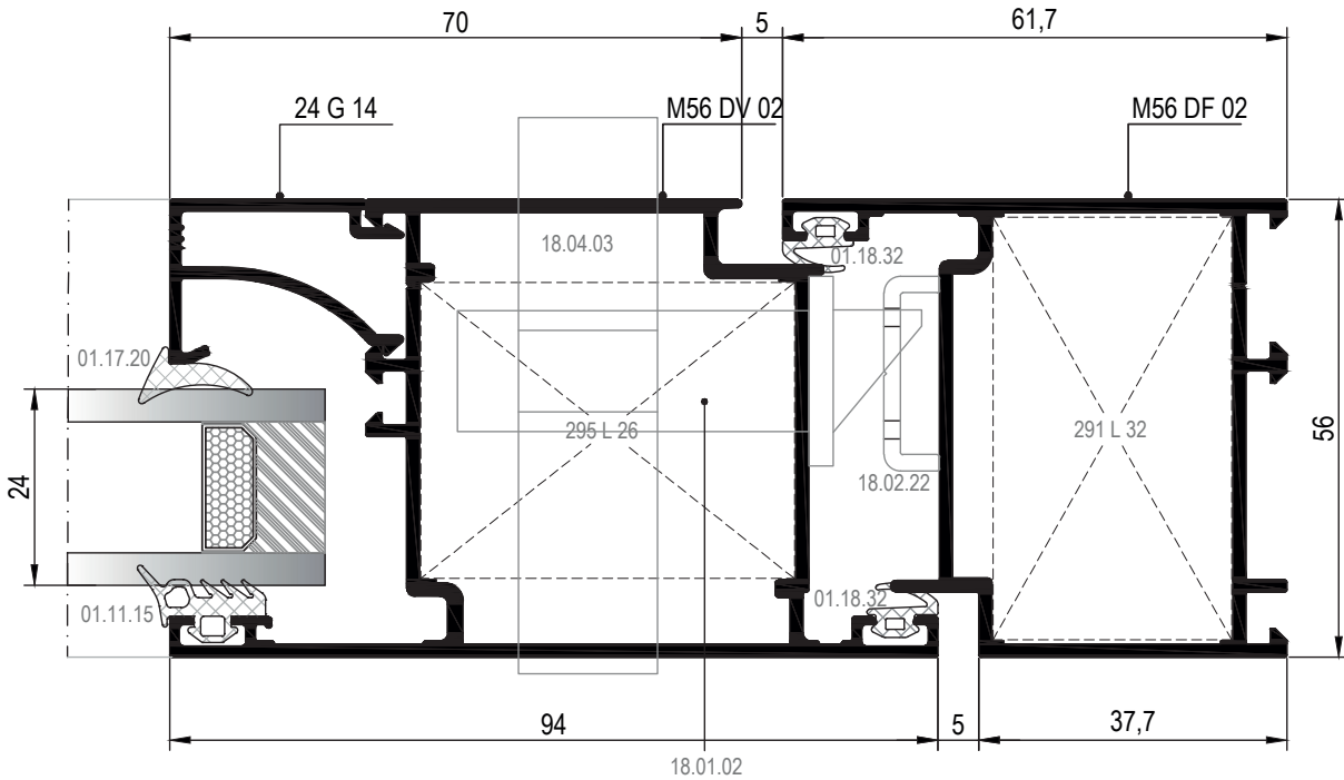
32 DETAYI DETAIL
