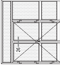
İÇE AÇILIM ADAPTÖRLÜ HEMİYÜZ KAPI DETAYLARI INWARD OPENING FLUSH DOOR DETAILS WITH ADAPTER
