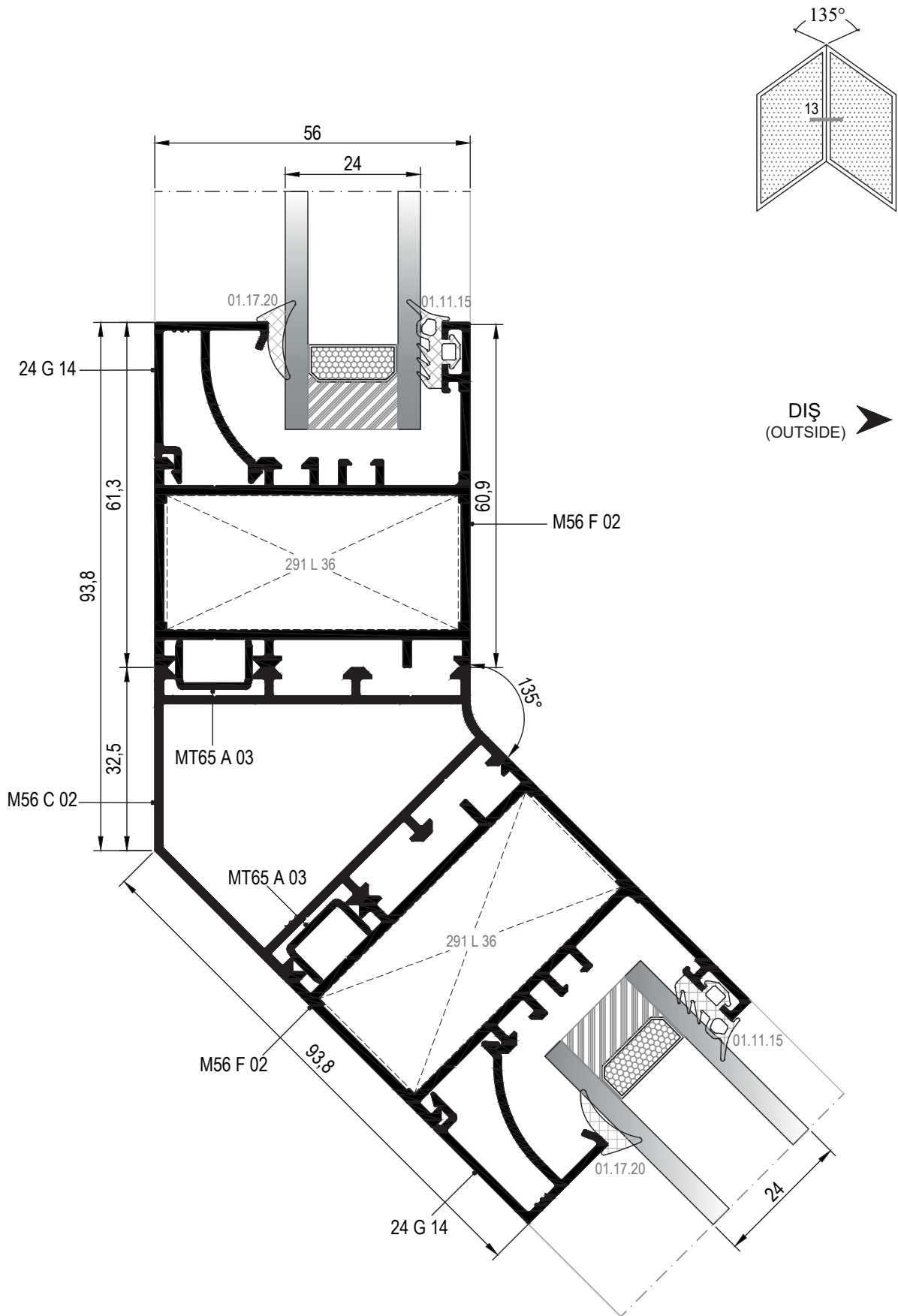
13 DETAYI DETAIL
